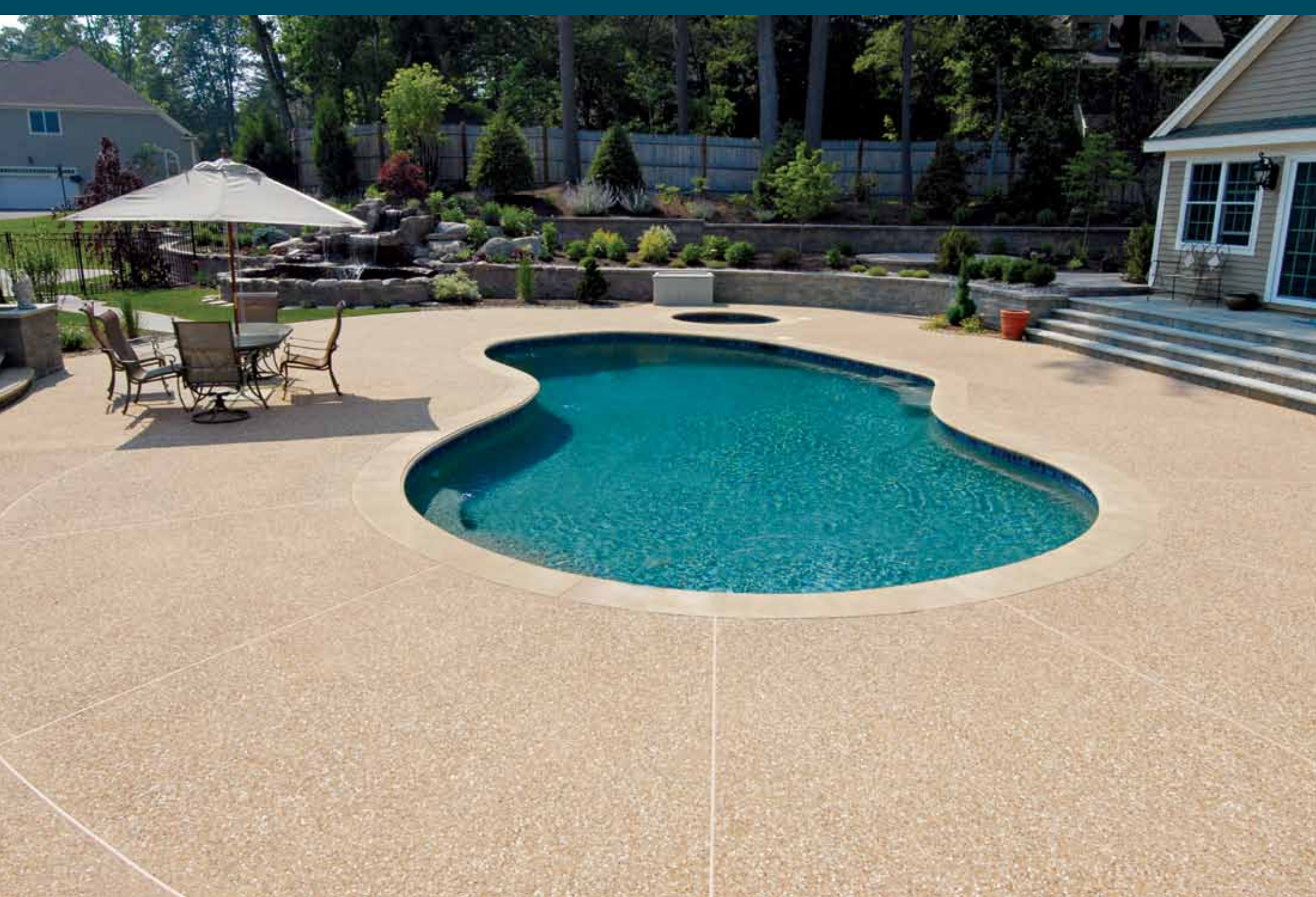
28 Exposed aggregate pool deck , cantilever coping band, block walls, limestone steps, water feature
